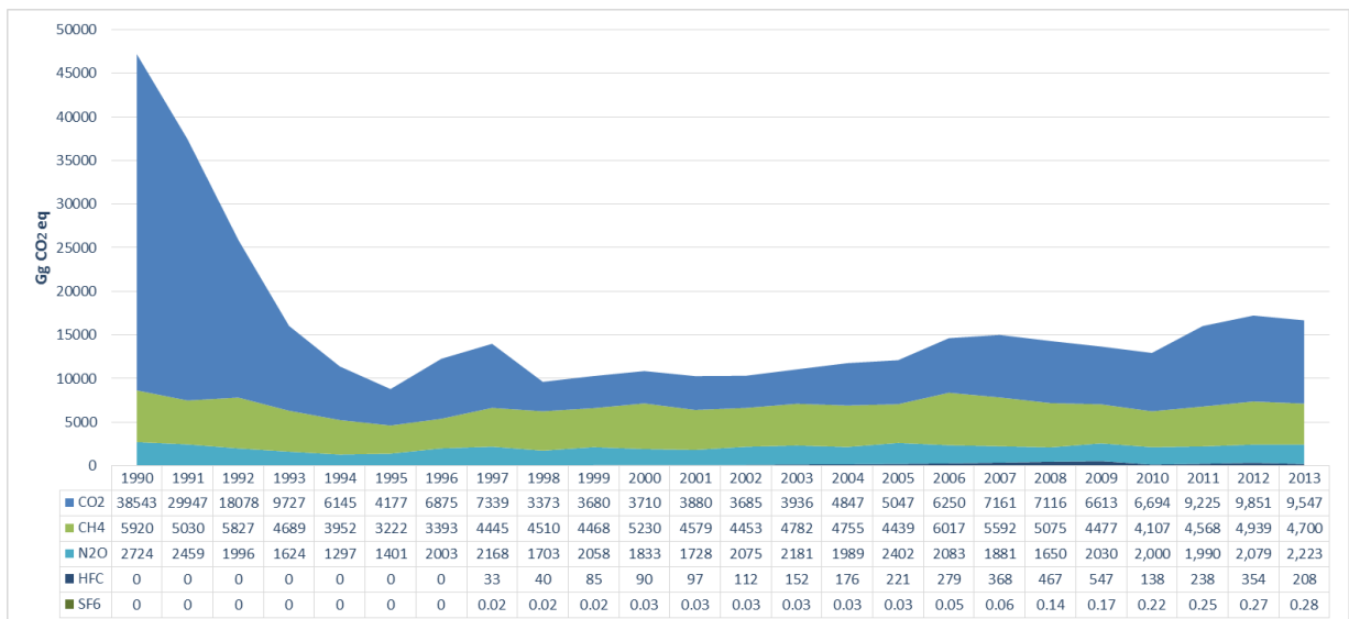
Figure 3.3 - GHG EMISSION TRENDS IN GEORGIA IN 1990-2013 (Gg CO 2 -eq.)
