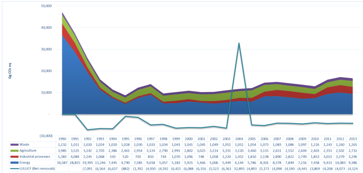
Figure 3.2 - GHG EMISSION TRENDS IN GEORGIA BY SECTORS IN 1990-2013 (Gg CO 2 -eq.)
