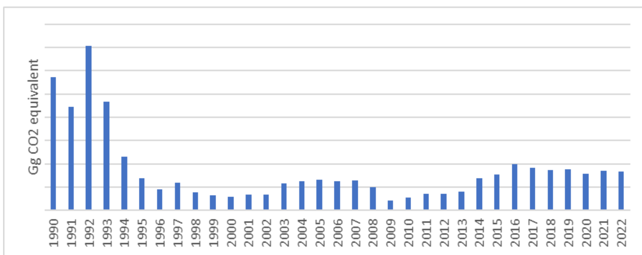
FIGURE 4-6. CO 2 - OF EMISSIONS FROM GLASS PRODUCTION ( GG ) 1990-2022
