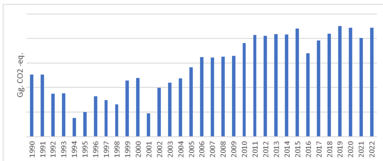
FIGURE 4-10. N 2 O EMISSIONS FROM NITRIC ACID PRODUCTION (GG) 1990-2022
