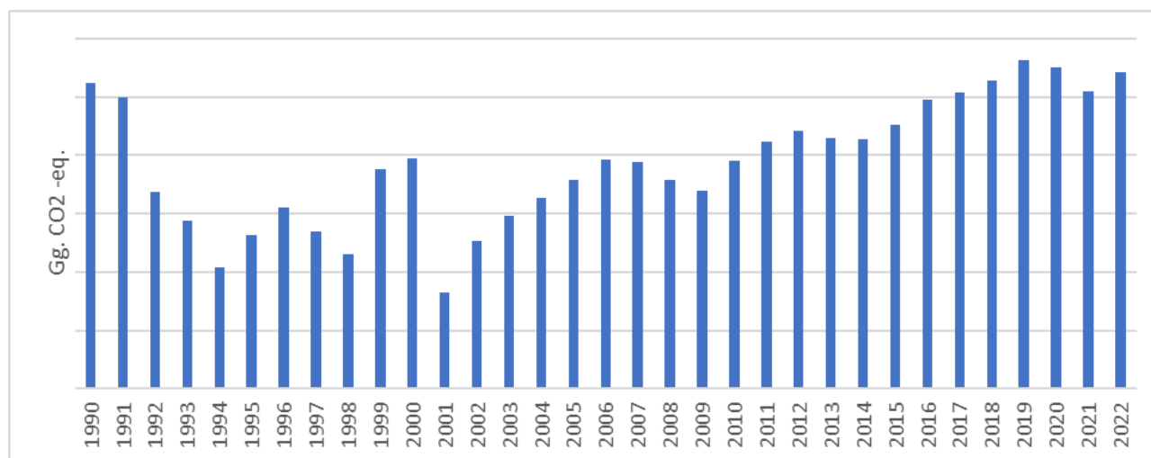
FIGURE 4-9. CO 2 EMISSIONS FROM AMMONIA PRODUCTION (GG) 1990-2022
