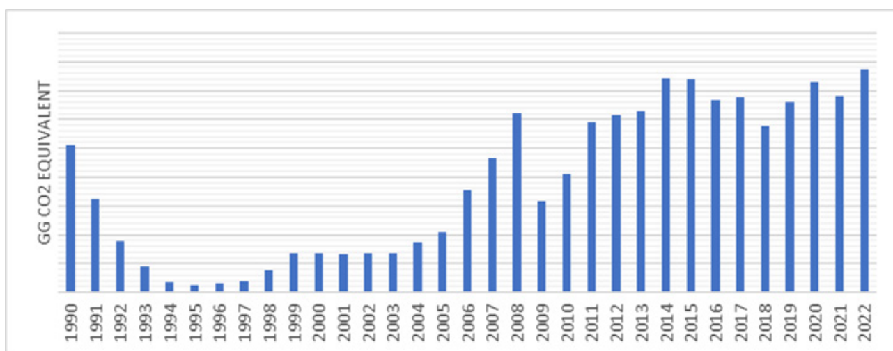
FIGURE 4-2. CO 2 EMISSIONS FROM CEMENT PRODUCTION (GG) 1990 – 2022
